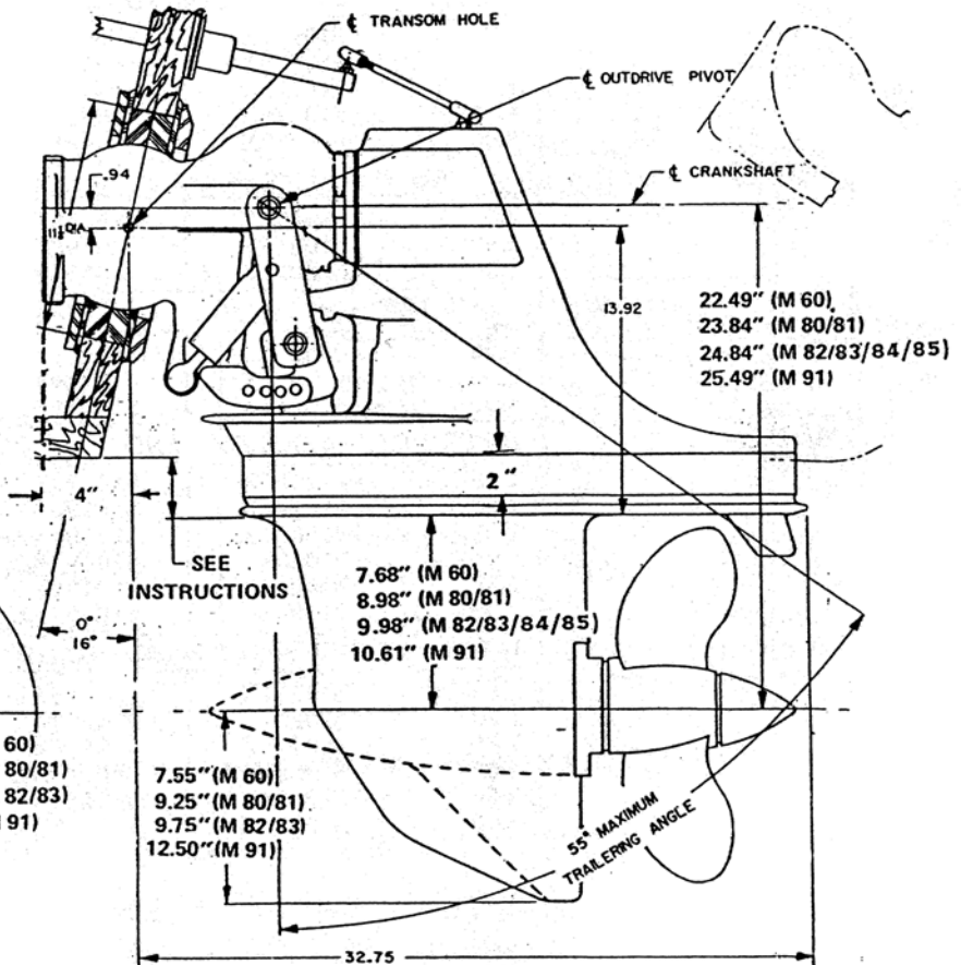
TYPE B UPPER HOUSING WITH BUILT-IN TWO INCH EXTENSION - SHIELDED BOOT FORM
