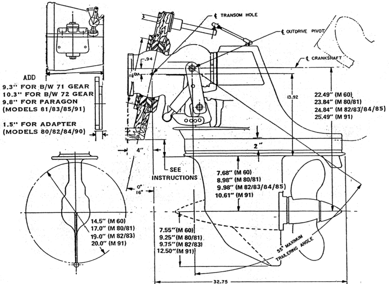
TYPE B UPPER HOUSING WITH BUILT-IN TWO INCH EXTENSION - SHIELDED BOOT FORM
